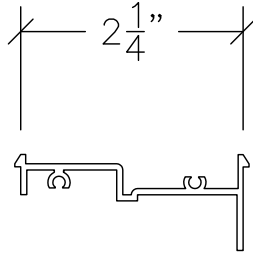
#214 HEAD
