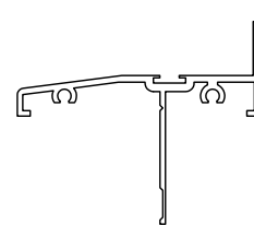
#270 SILL
