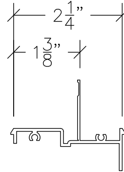
#271 HEAD
