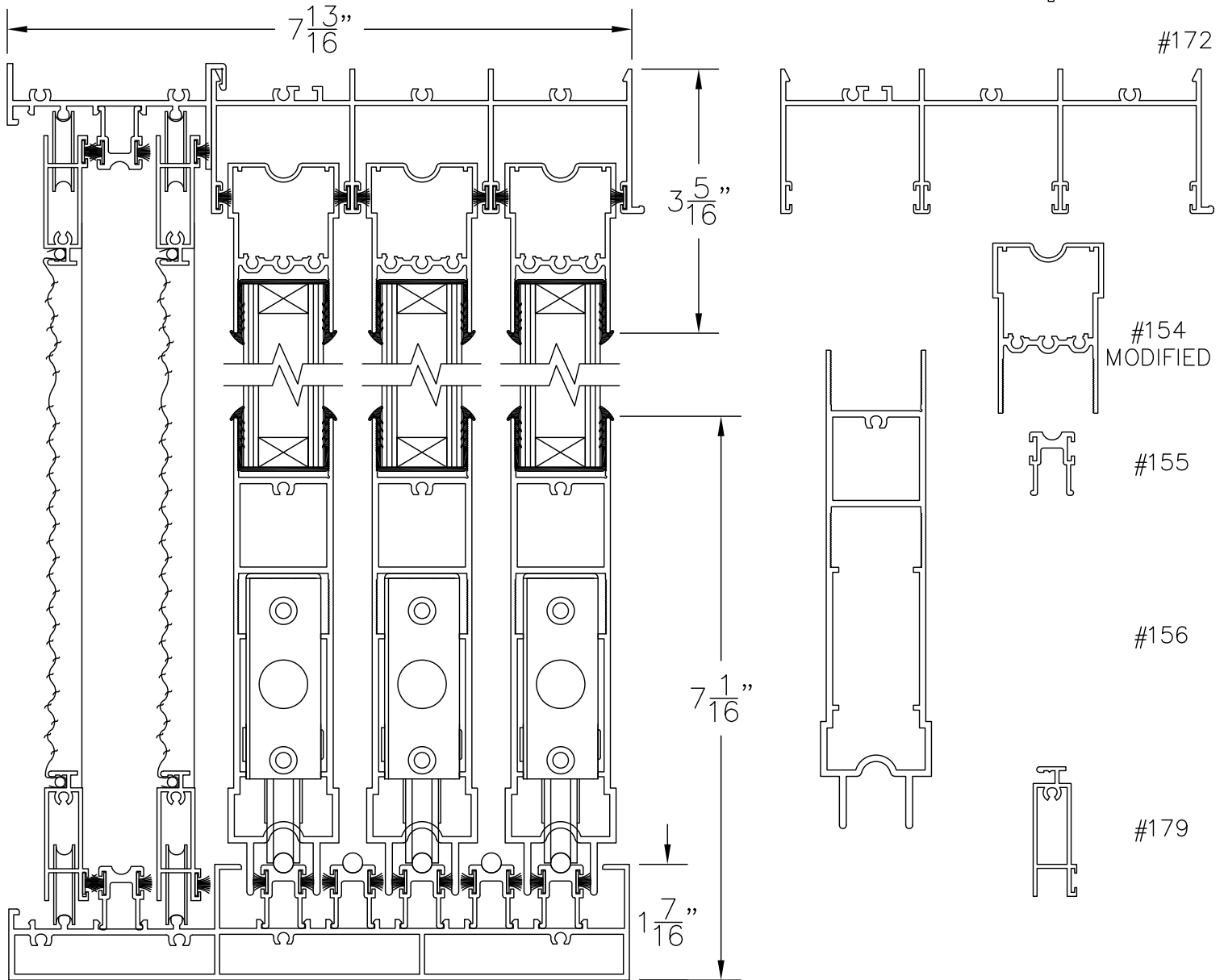
① MULTI-SLIDING GLASS DOOR HEAD + 190 SCREEN TRACK
