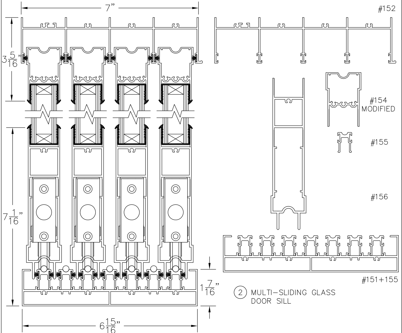
① MULTI-SLIDING GLASS DOOR HEAD
