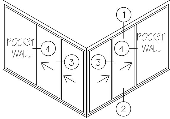
270° P4XP MULTI-SLIDING GLASS DOOR EXTRUSIONS - POCKET DOUBLE GLAZED SCALE: 1:8
