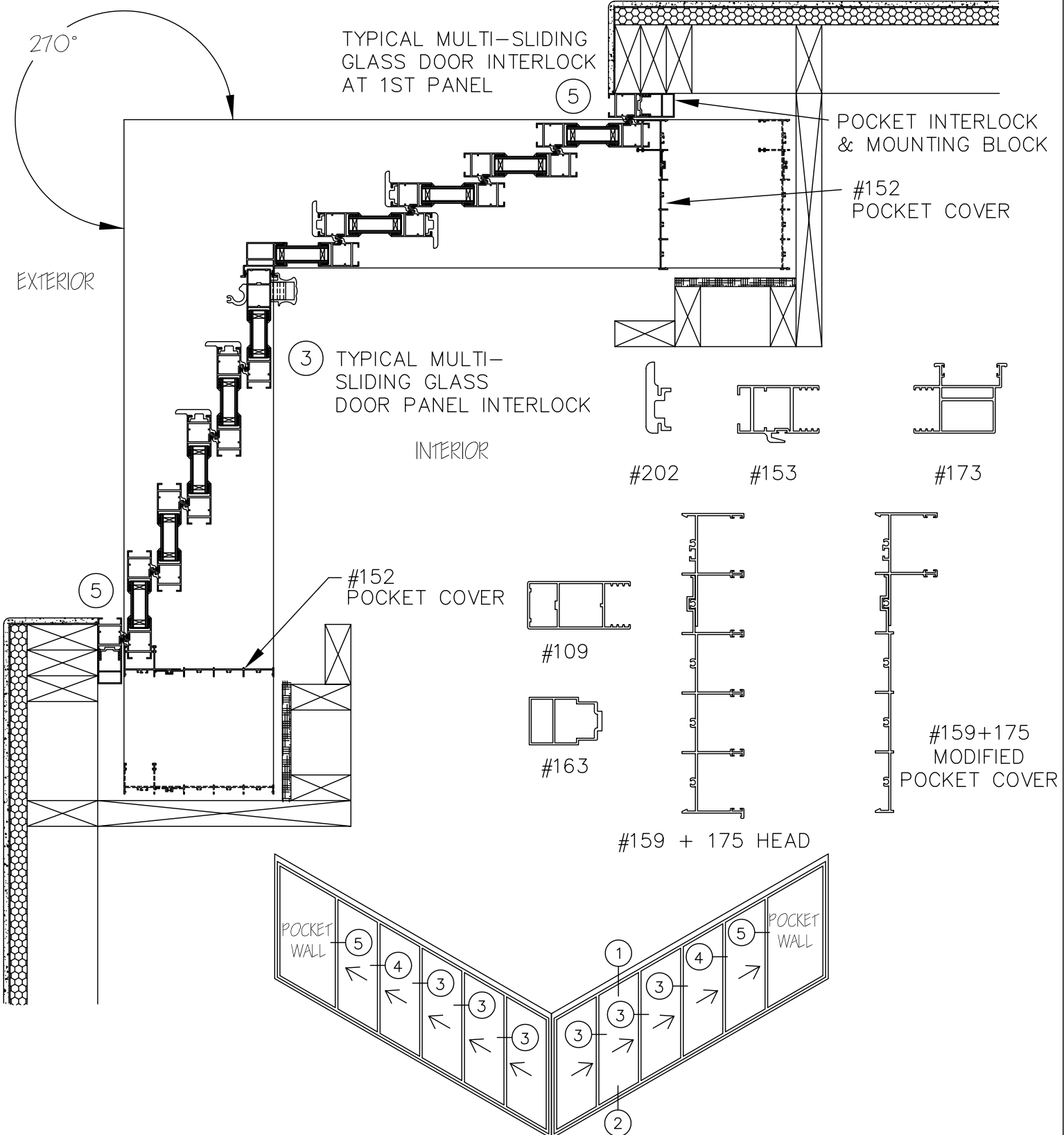
270° P10XP MULTI-SLIDING GLASS DOOR EXTRUSIONS - POCKET DOUBLE GLAZED SCALE: 1:8
