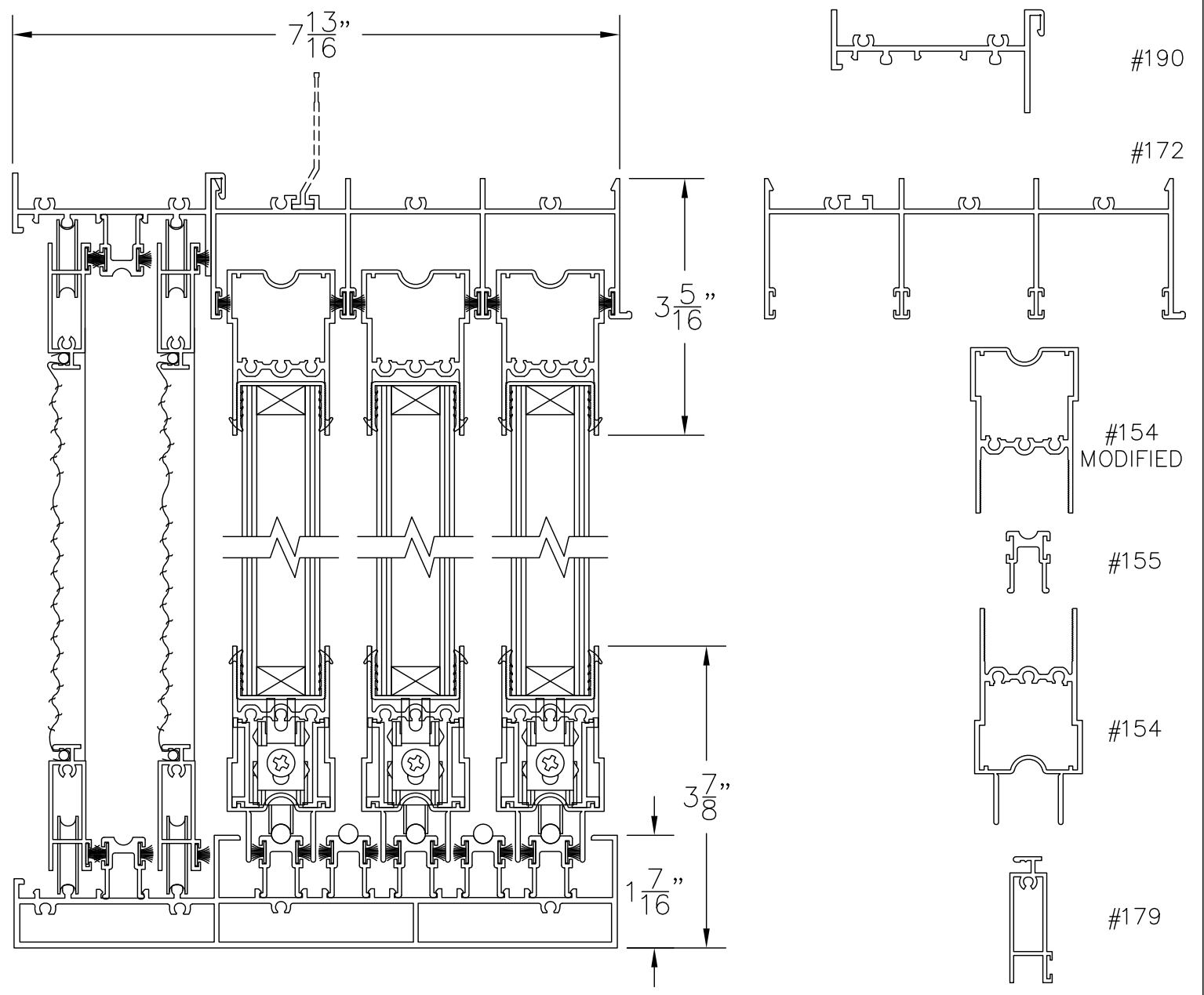
① MULTI-SLIDING GLASS DOOR HEAD + 190 SCREEN TRACK
