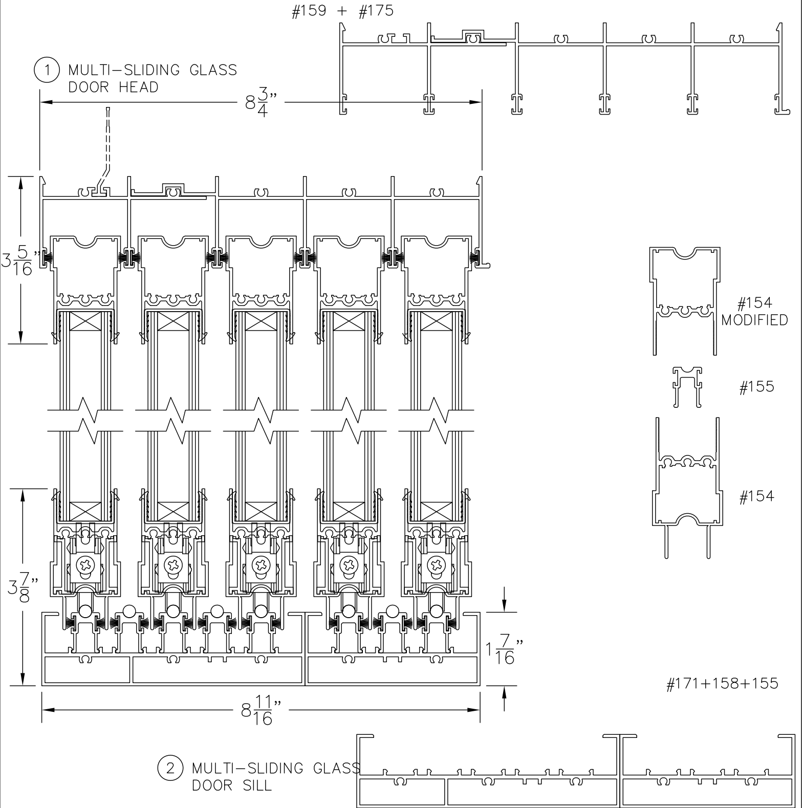
VERTICAL SECTION THROUGH MULTI-SLIDING GLASS DOOR DOUBLE GLAZED SCALE: 1:2
