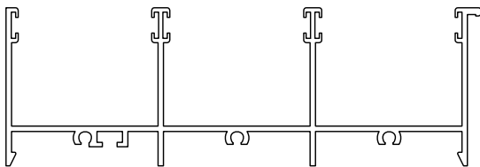
#172 HEAD/JAMB
