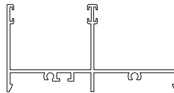
POCKET COVER
