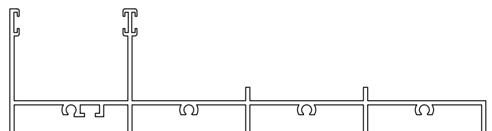
POCKET COVER
