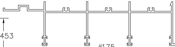
#175 HEAD/JAMB EXTENSION
