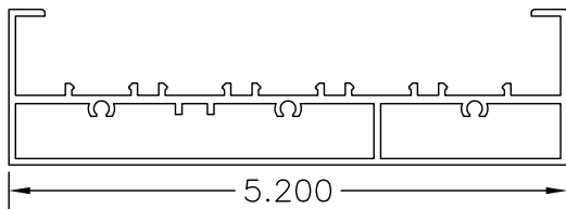
#171 SILL
