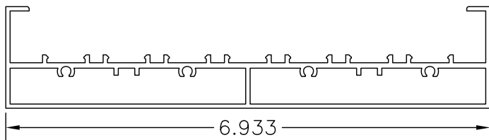
#151 SILL
