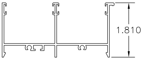
#159 HEAD/JAMB
