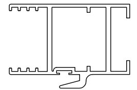
#153 INTERLOCK STILES
