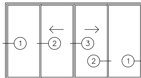
HORIZONTAL SECTION THROUGH 4 1/8" 4-PANEL – SGD3 / SGD4 SLIDING GLASS DOOR – DOUBLE GLAZED
