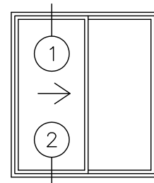
VERTICAL SECTION THROUGH SGD @ SILL COVER – SGD3 DOUBLE GLAZED
