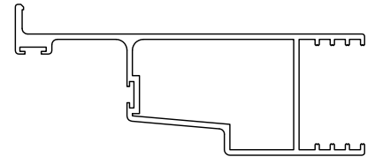
#131 LOCKSTILE OXO
