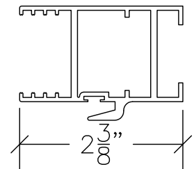
#153 INTERLOCKER
