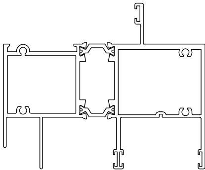
#1439 WINDOW WALL SILL/SLIDING GLASS DOOR HEAD USED FOR TRANSOM WINDOW OVER SLIDING GLASS DOOR APPLICATIONS
