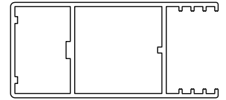
#109 LEAD STILE AND FIXED BACK STILE
