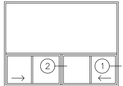
HORIZONTAL SECTION THROUGH 4 1/8" PERIMETER FRAME & STRUCTURAL MUNTIN W/ HORIZONTAL SLIDER INSERT DOUBLE GLAZED SCALE: HALF SIZE
