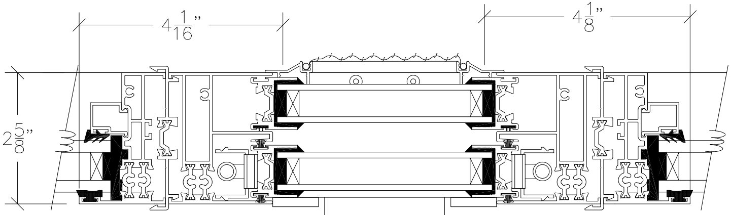
① SINGLE HUNG JAMB
