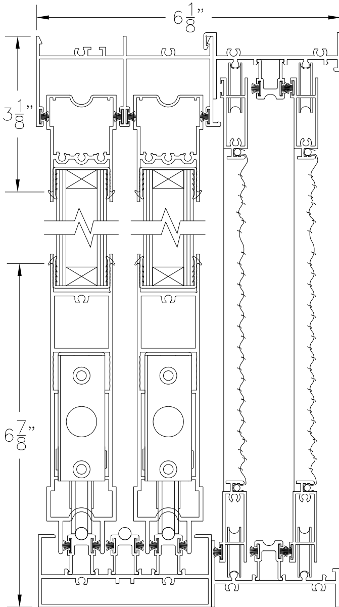
② MULTI-SLIDING GLASS DOOR SILL + 190 (WITH SCREENS)
