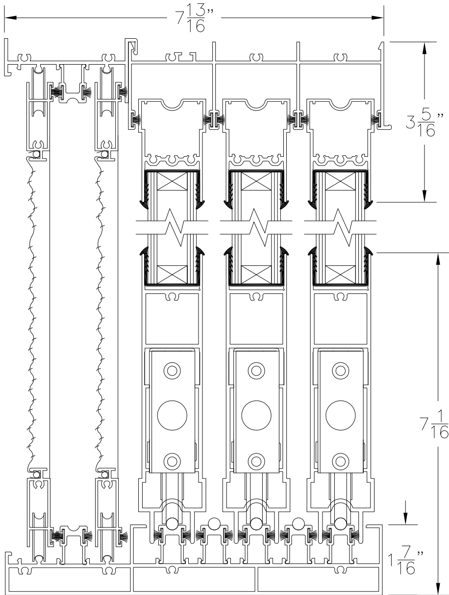
① MULTI-SLIDING GLASS DOOR HEAD + 190 SCREEN TRACK
