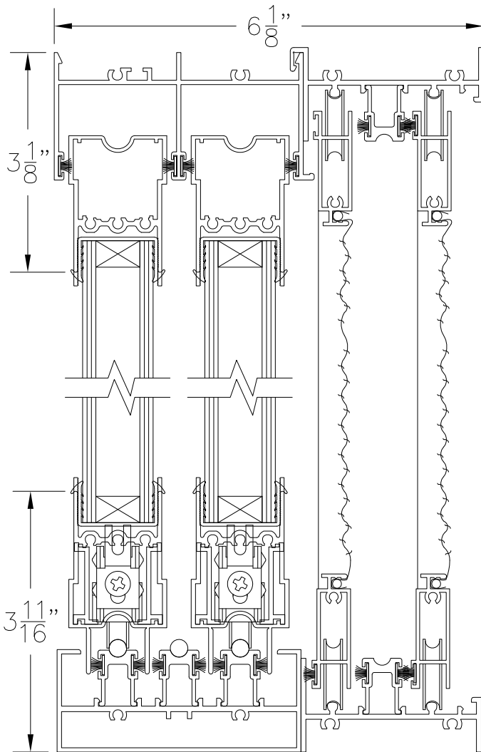
① MULTI-SLIDING GLASS DOOR HEAD + 190 SCREEN TRACK
