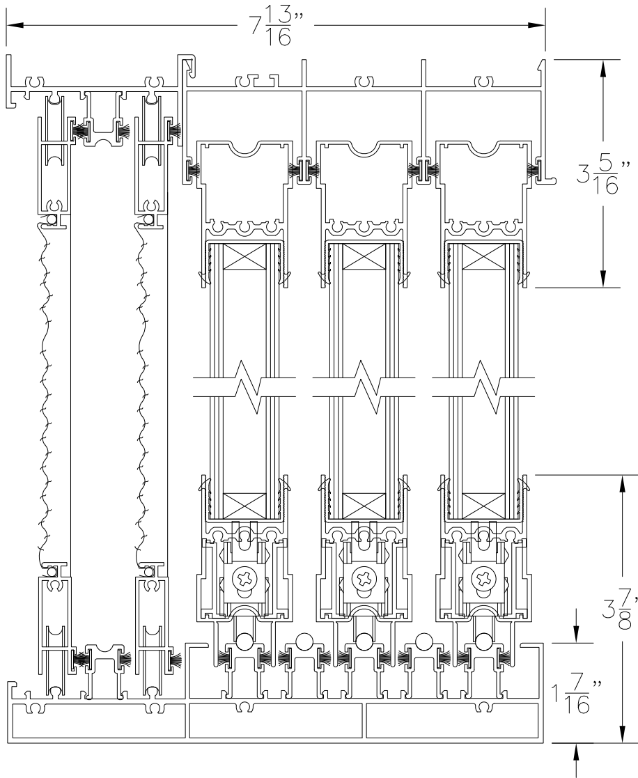
① MULTI-SLIDING GLASS DOOR HEAD + 190 SCREEN TRACK
