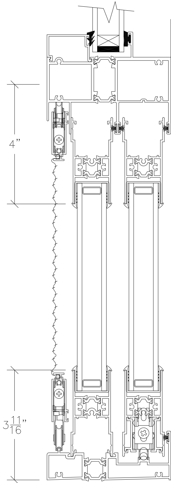
VERTICAL SECTION THROUGH THERMAL BREAK SLIDING GLASS DOOR W/TRANSOM DOUBLE GLAZED
