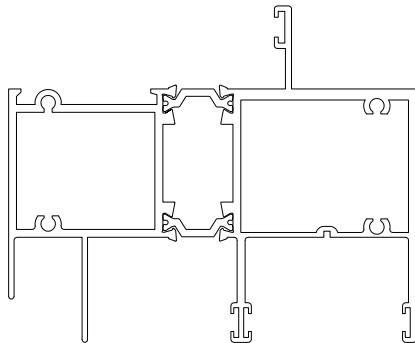
#1439 WINDOW WALL SILL/SLIDING GLASS DOOR HEAD USED FOR TRANSOM WINDOW OVER OVER SLIDING GLASS DOOR APPLICATIONS
