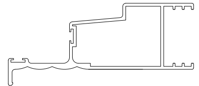
#131 LOCKSITLE OXXO
