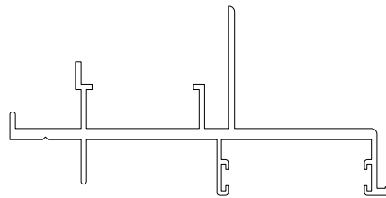
#119 OXXO ADAPTOR
