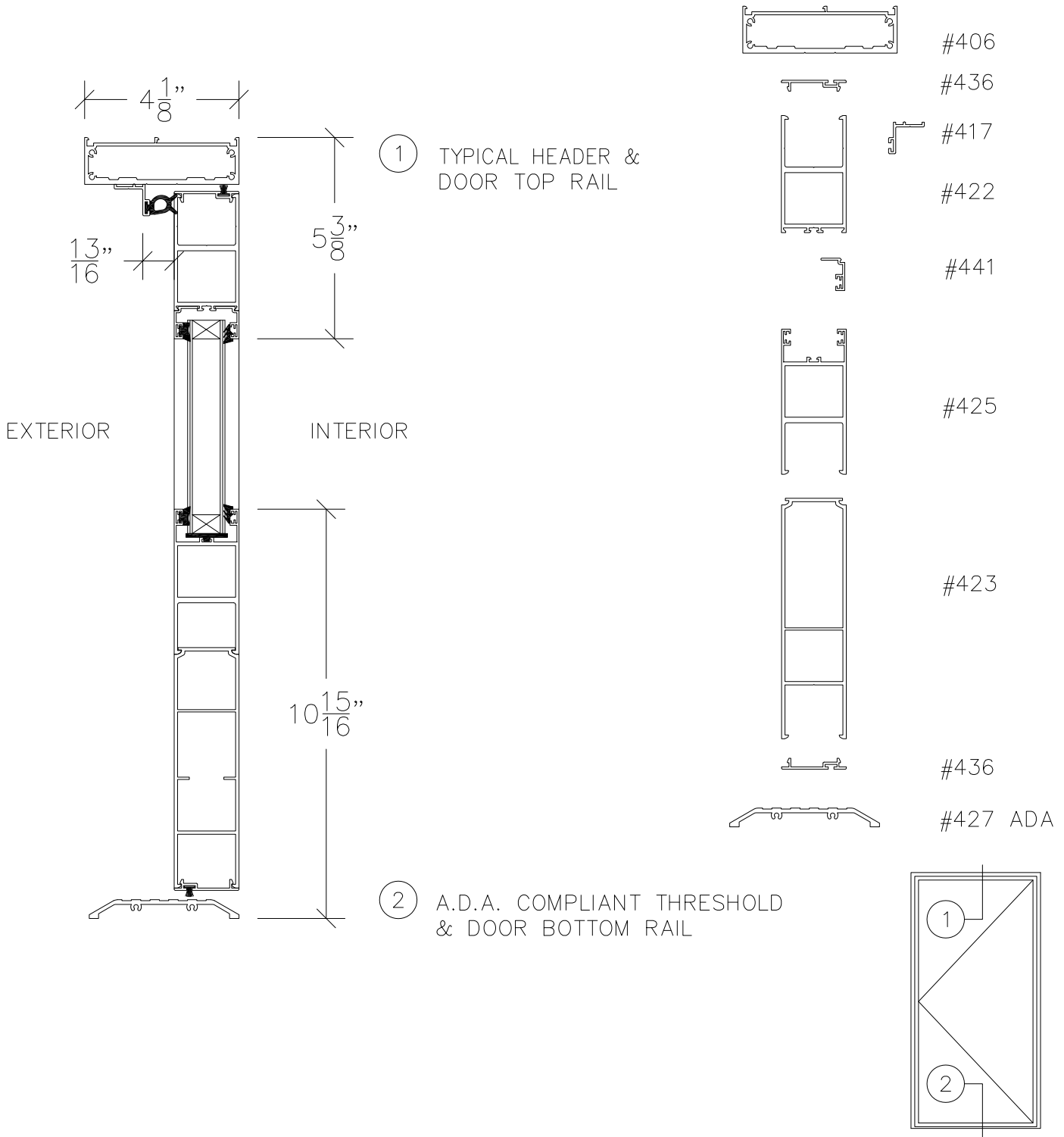
VERTICAL SECTION THROUGH SINGLE/PAIR SWINGING DOORS SCALE: QUARTER SIZE
