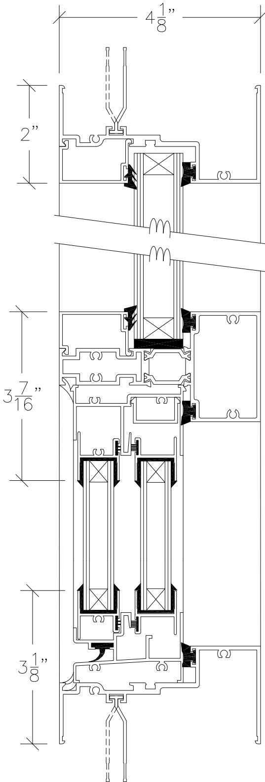
4 1/8" PERIMETER FRAME & MUNTIN DETAIL W/ HORIZONTAL SLIDER INSERT - DOUBLE GLAZED SCALE: HALF SIZE
