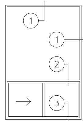
4 1/8" PERIMETER FRAME & MUNTIN DETAIL W/ HORIZONTAL SLIDER INSERT - DOUBLE GLAZED SCALE: HALF SIZE
