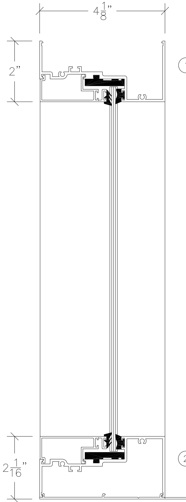
SUB SILL DETAIL - SINGLE GLAZED SCALE: HALF SIZE
