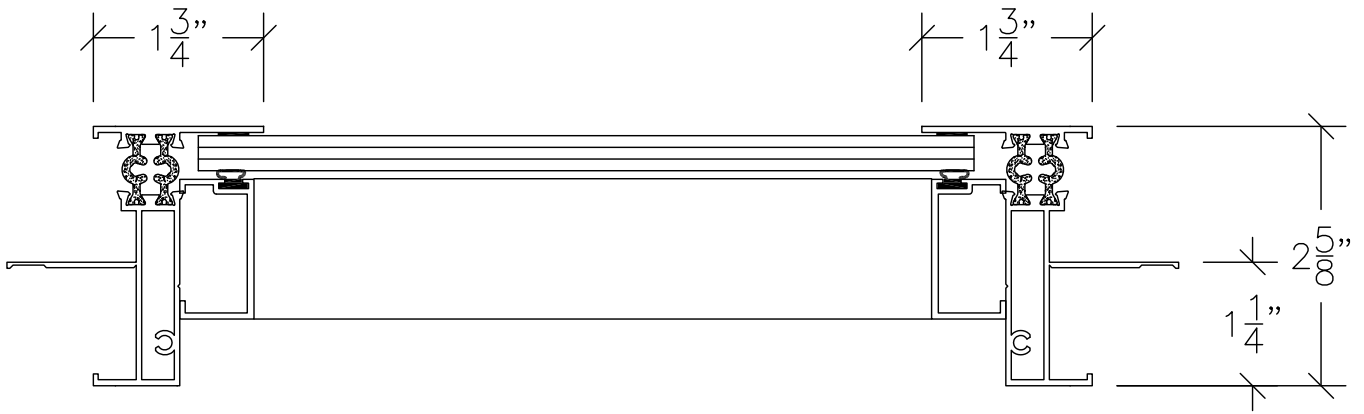
① TYPICAL PERIMETER FRAME
