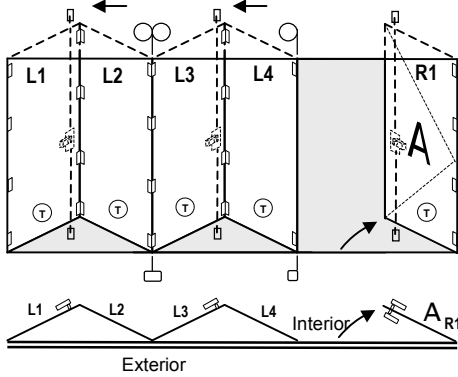
4L1RSIFD1DG
