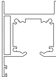
#700 HEAD
