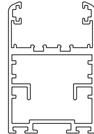
#701 PANEL
