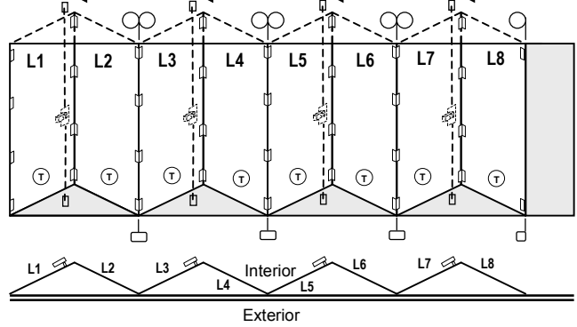
8LSIFD1DG
