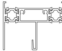
② HORIZONTAL MULLION
