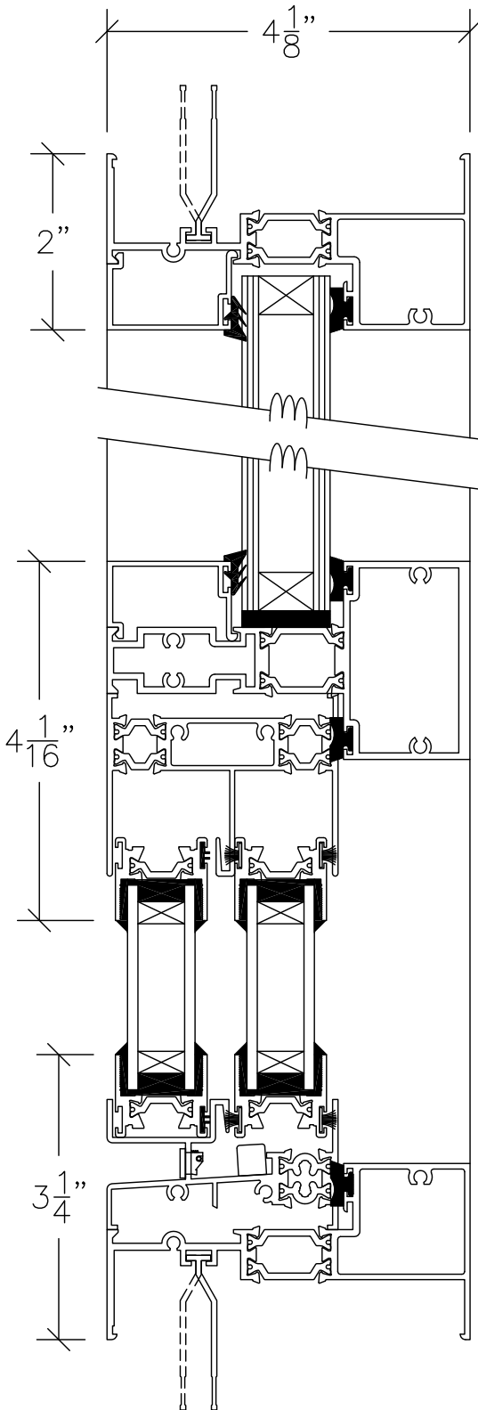
① PERIMETER FRAME HEAD/JAMB
