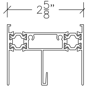
#1251 HEAD
