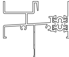
#1250 SILL
