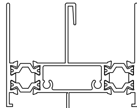
#1251 HEAD
