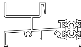
#1250 SILL
