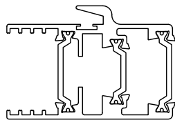
#1156 INTERLOCK STILES
