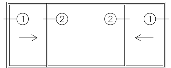
HORIZONTAL SECTION THROUGH HORIZONTAL SLIDER DOUBLE GLAZED SCALE: QUARTER SIZE
