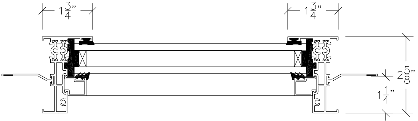
① TYPICAL PERIMETER FRAME
