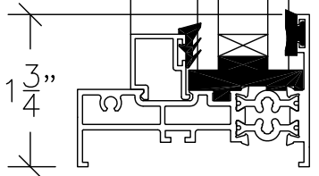
① TYPICAL PERIMETER FRAME
