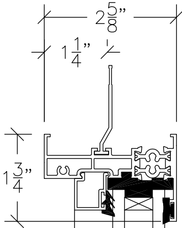
① TYPICAL PERIMETER FRAME
