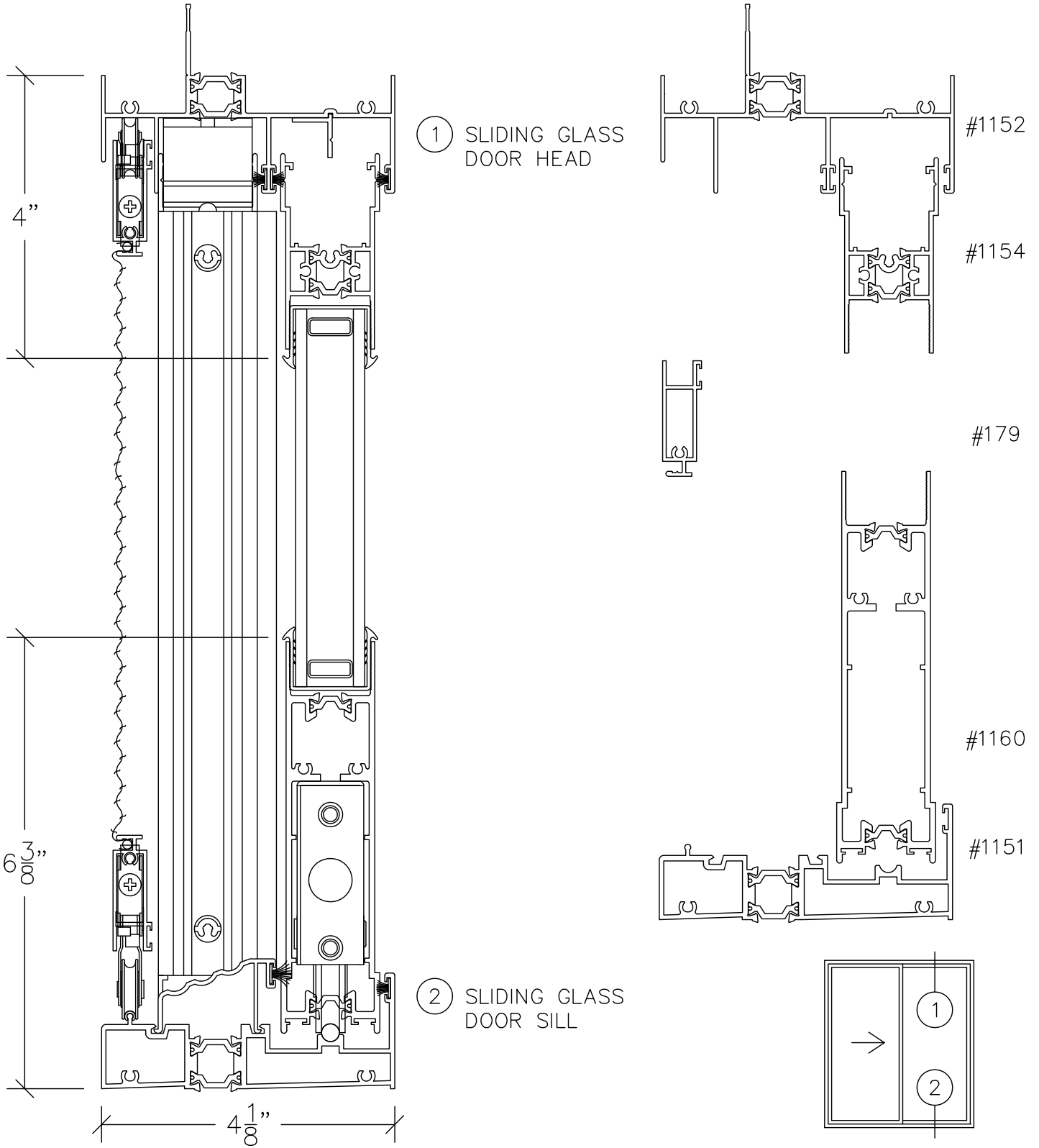
VERTICAL SECTION THROUGH THERMAL BREAK TSGD4 @ SILL COVER DOUBLE GLAZED
