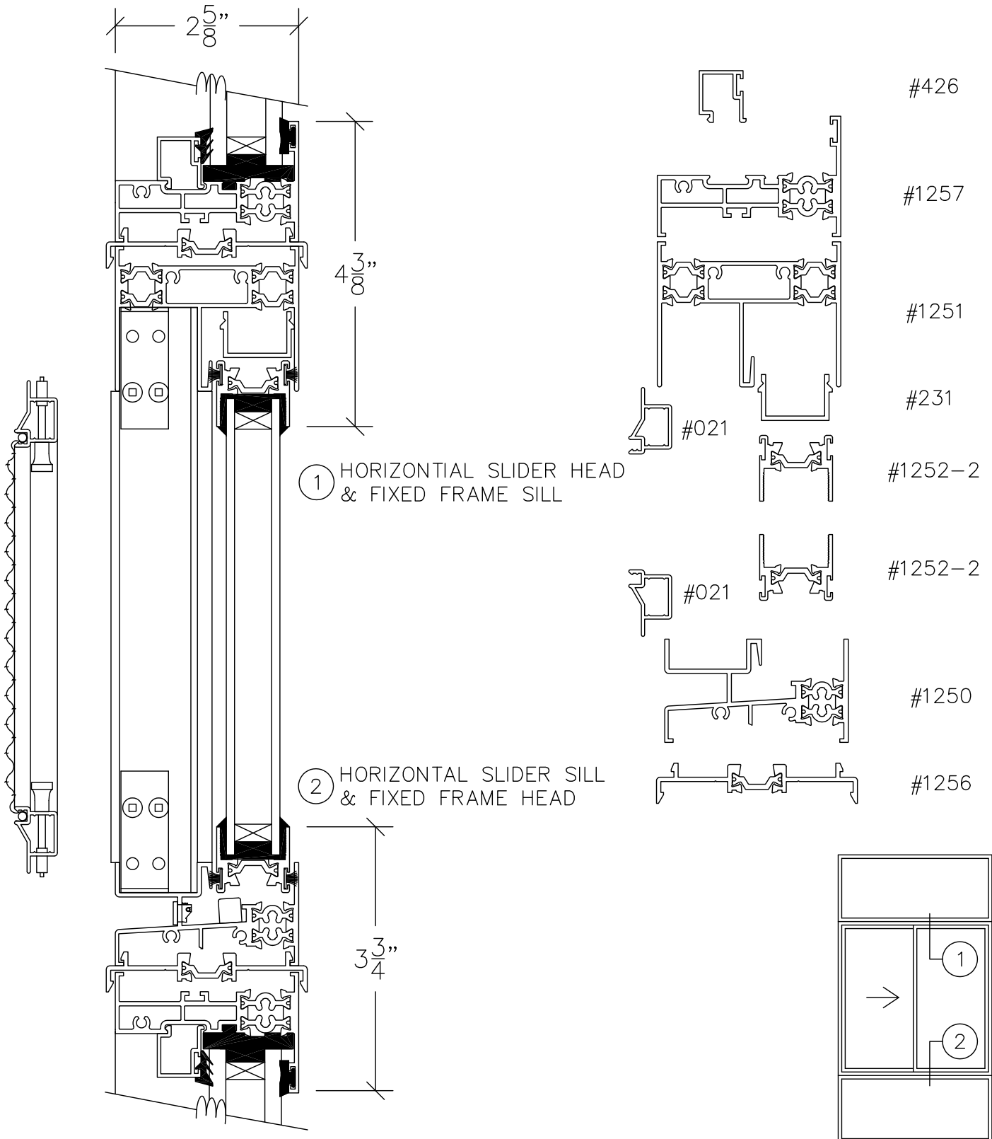
VERTICAL SECTION THROUGH HORIZONTAL SLIDER STACK DOUBLE GLAZED SCALE: HALF SIZE
