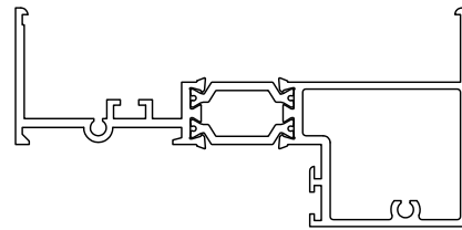
① TYPICAL PERIMETER FRAME
